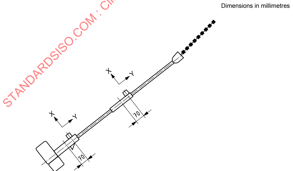
Figure C.4 — Example of transducer location/orientation (long-reach hedge trimmers)
