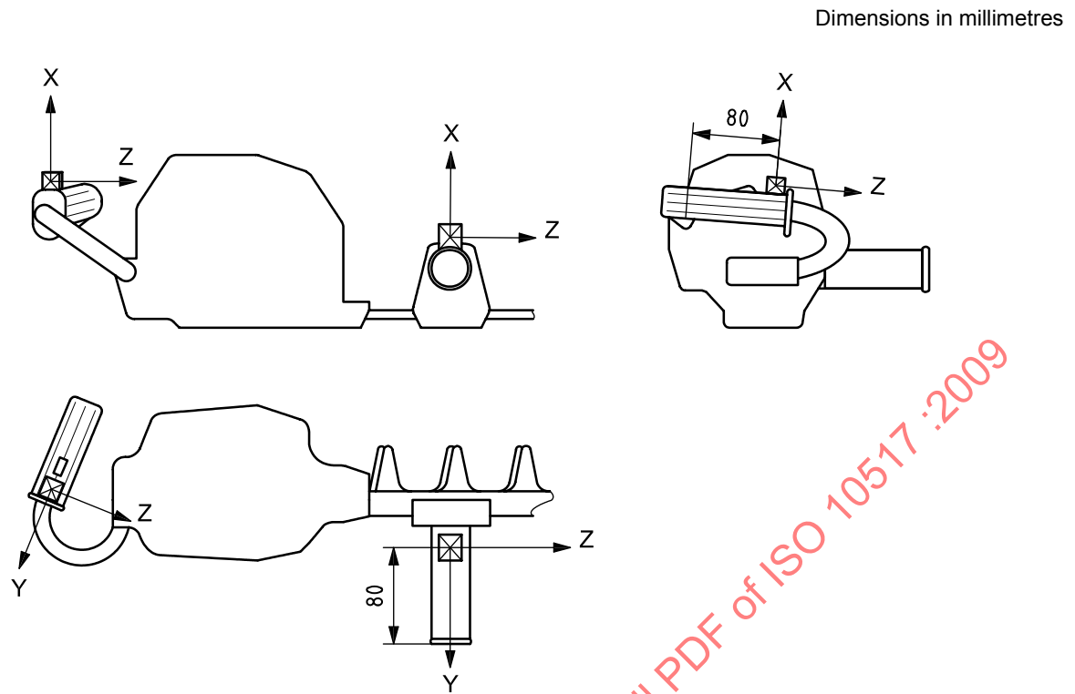
Figure C.3 — Example of transducer location/orientation (lateral rear handle)
