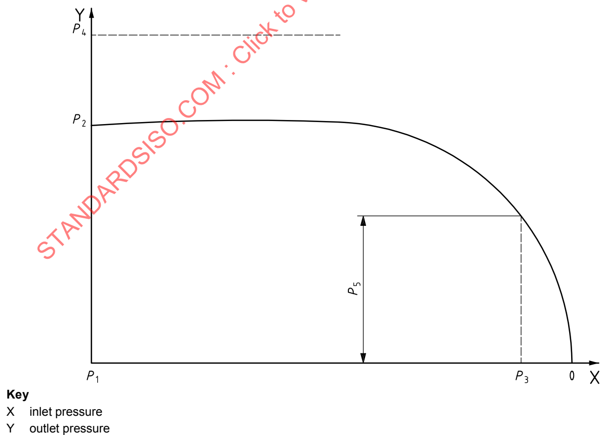
Figure 4 — Typical falling pressure characteristic
