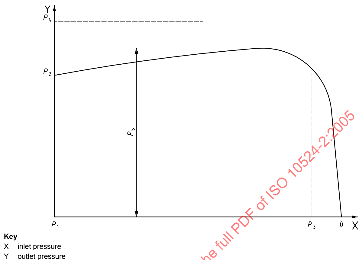
Figure 3 — Typical rising pressure characteristic
