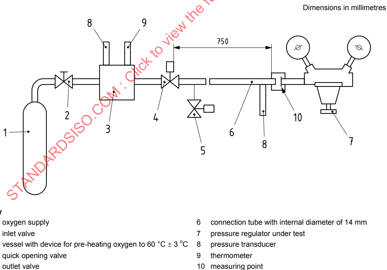
Figure 5 — Test bench for ignition test on manifold pressure regulators
