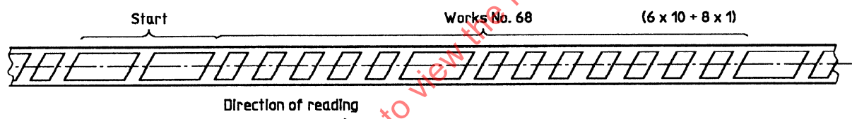
Figure A.2 — Example of identification of manufacturer on indented wire
