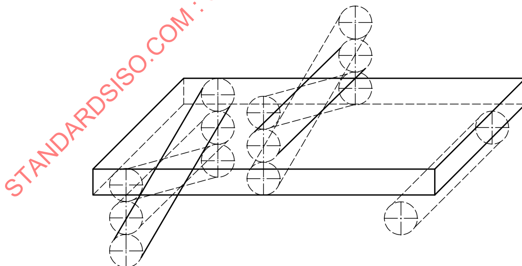
Figure 2 — Allowable movement of rods
