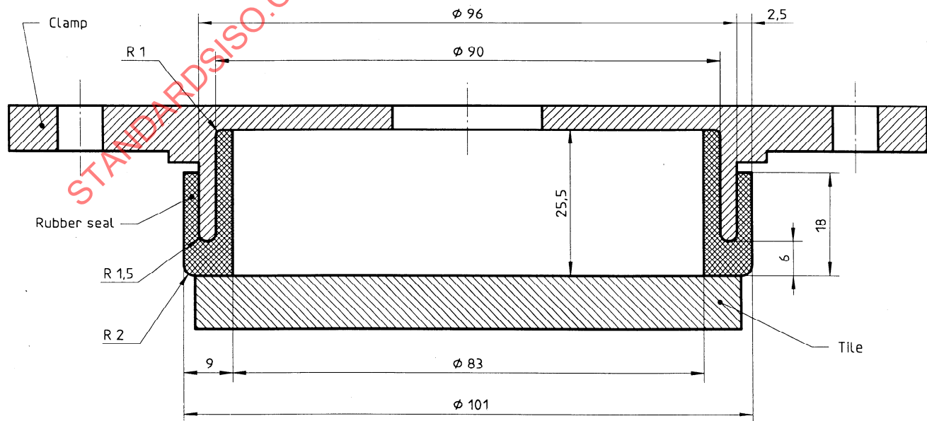
Figure 2 — Specimen holder
