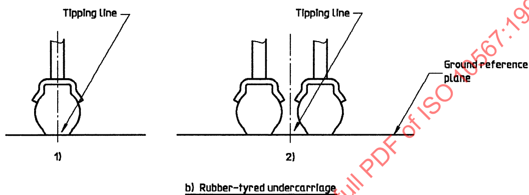
Figure 4 — Tipping lines
