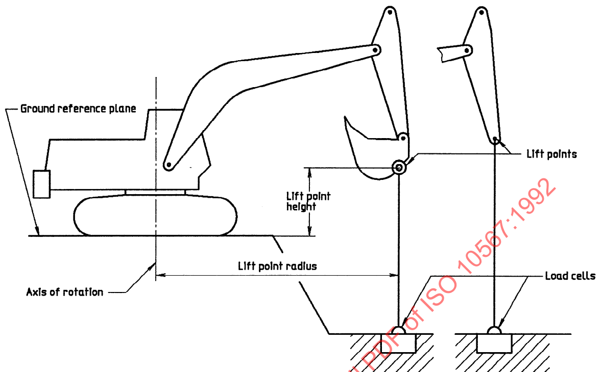
Figure 6 — Fixed dead weight
