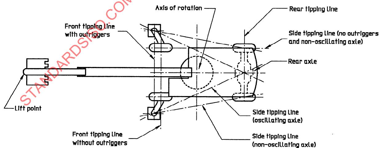
Figure 3 — Rubber-tyred undercarriage
