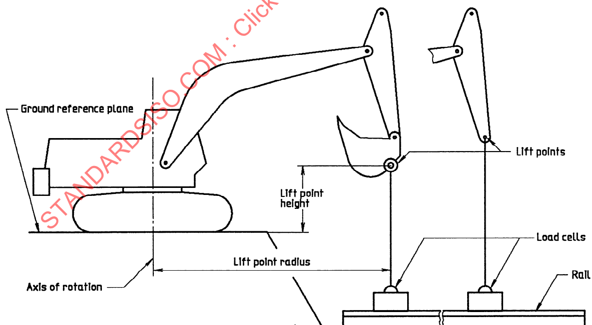
Figure 5 — Self-aligning dead weight
