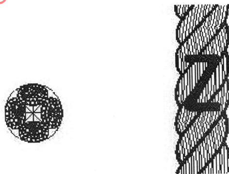
Figure 2 — Shape of a 4-strand shroud-laid rope (type B)
