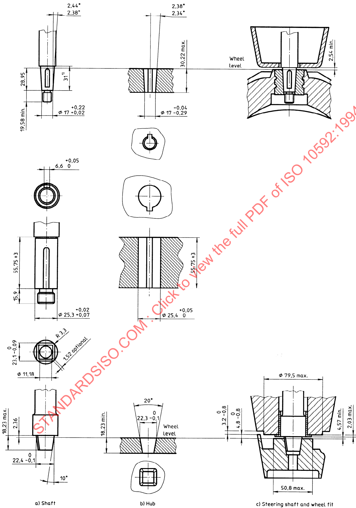
Figure 3 — Steering shafts and steering-wheel hubs
