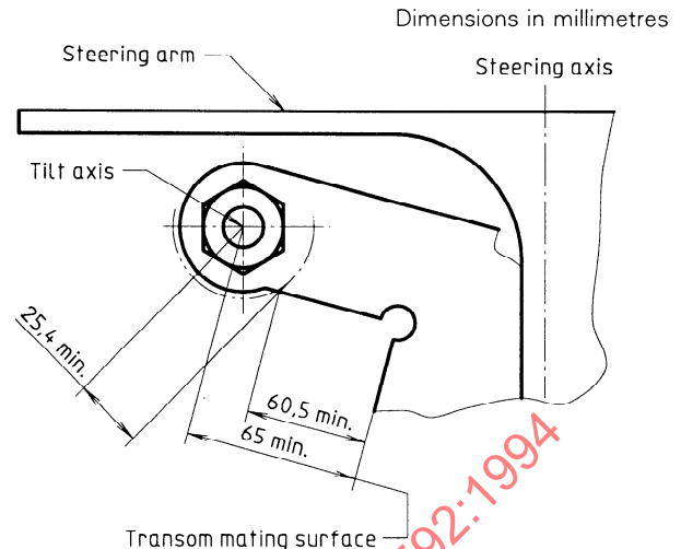
Figure 2 — Motor-mounted steering tilt axis
