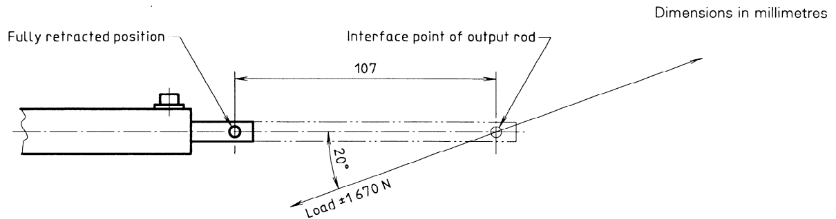
Figure 4 — Output ram fatigue test
