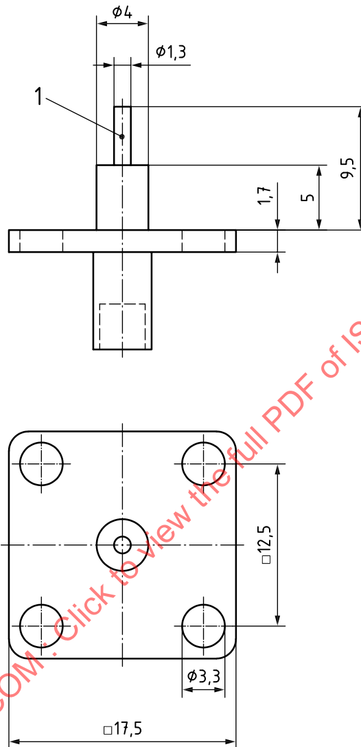
e) Sub miniature version A — Coaxial RF (SMA) connector
