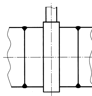
Figure 5 — Butt-welded ends
