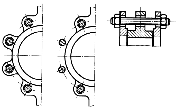
a) Valve with central lugs
