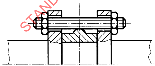
Figure 4 — Flangeless valve
