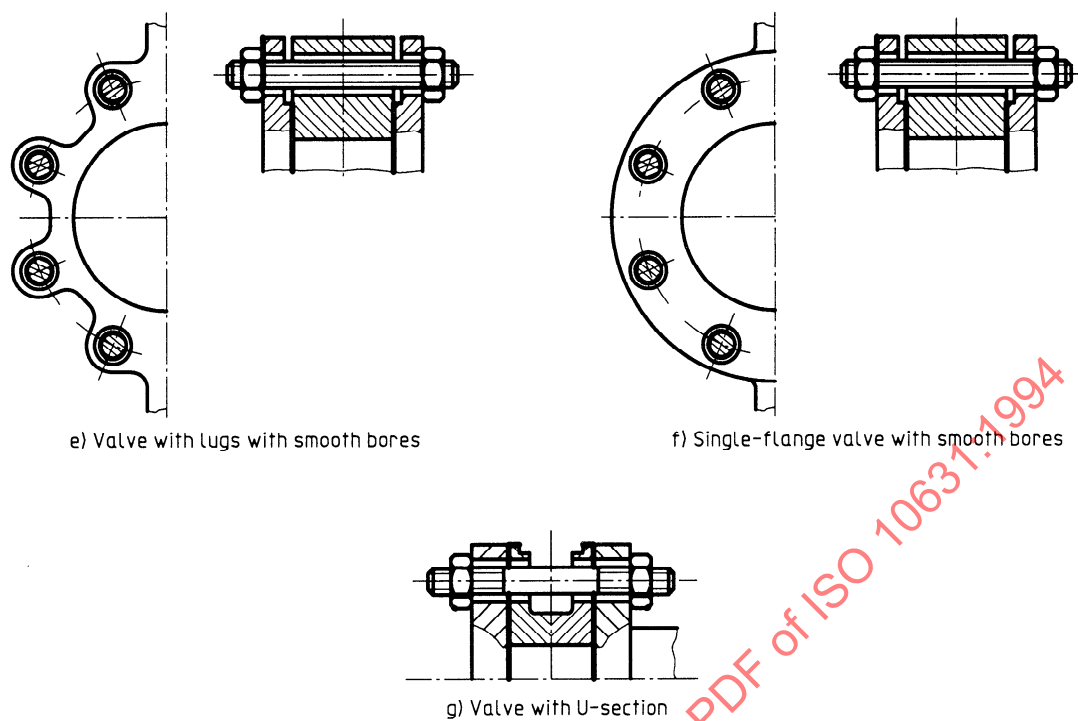
Figure 3 — Valves with lugs, single flange or with U-section
