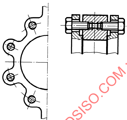
c) Valve with lugs with internally threaded bores
