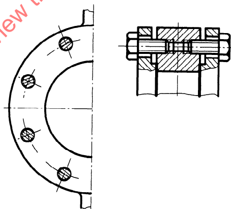
d) Single-flange valve with internally threaded bores
