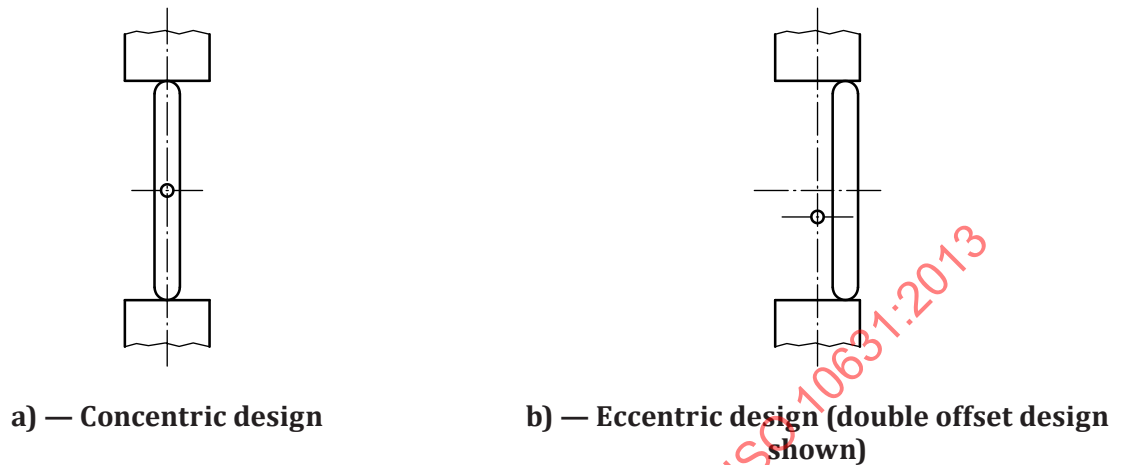
Figure 1 — Construction illustrations
