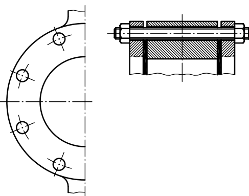
f) Single-flange valve with drilled holes
