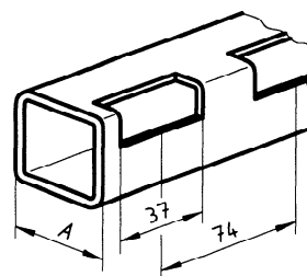
Square tubing profile 40 × 40 Rolled hollow section (RHS)
