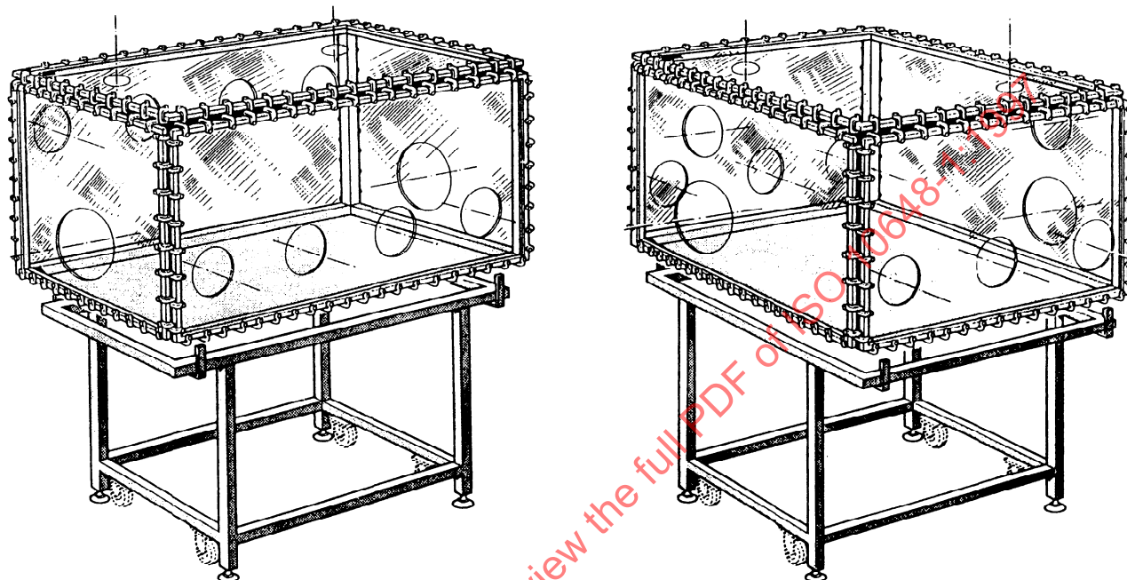
Figure 2 — Metal-framed containment enclosures (examples)
