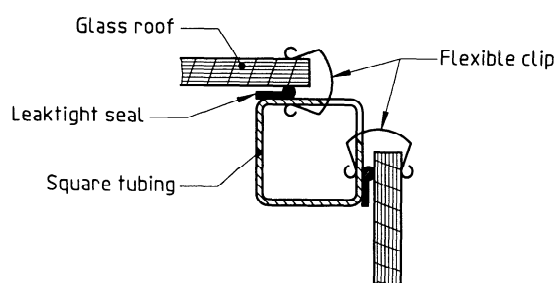
b) Detail of profiles (Ω or square tubing profile)
