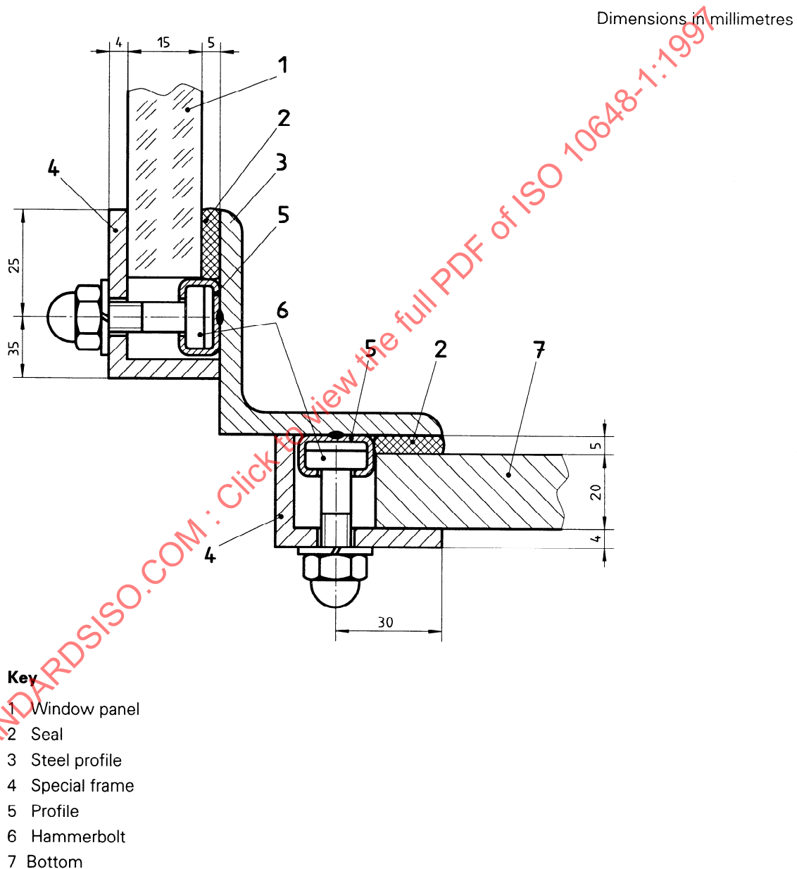
Figure 5 — Alternative principle of assembly and mounting of panels on metal-framed containment enclosures
