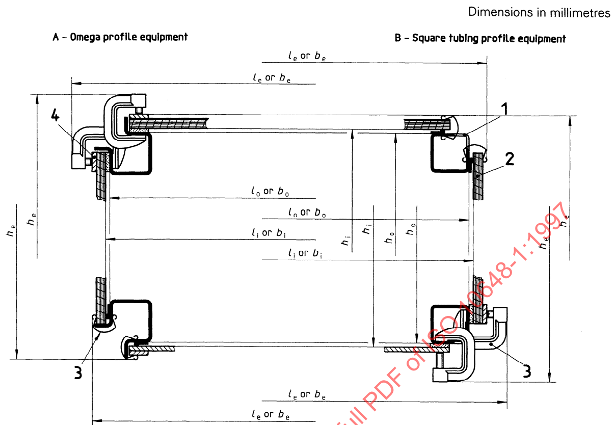
a) Description of assembly (with clamp or clip)
