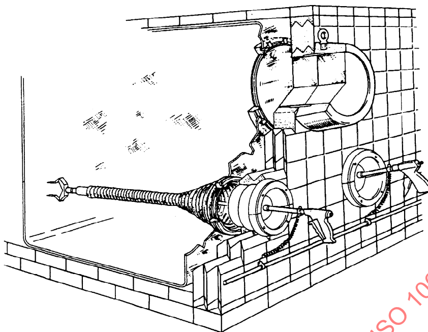
a) With lead bricks (see ISO 7212 and ISO 9404-1) and containment enclosure equipped with tongs.
