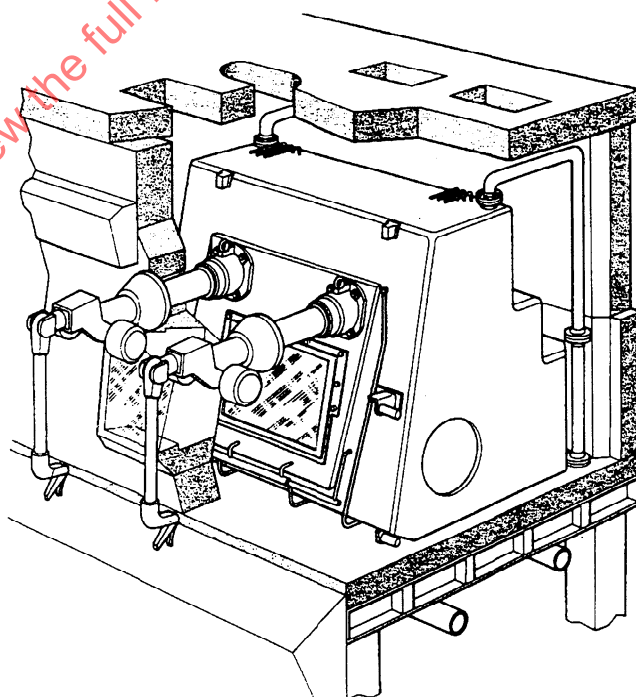
c) With cast iron, steel or lead panels and containment enclosure equipped with remote manipulators.
