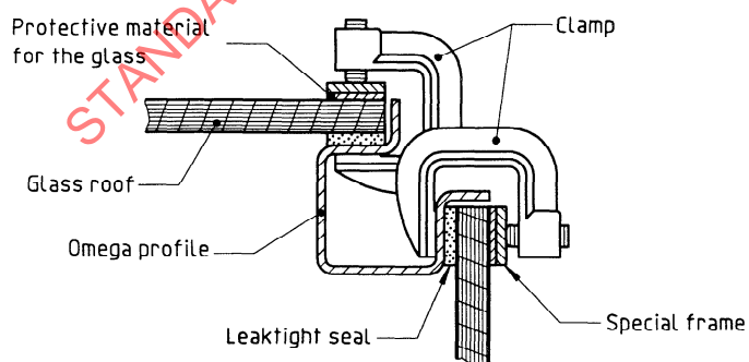
c) Detail of mounting on profile (with clamp or flexible clip)
