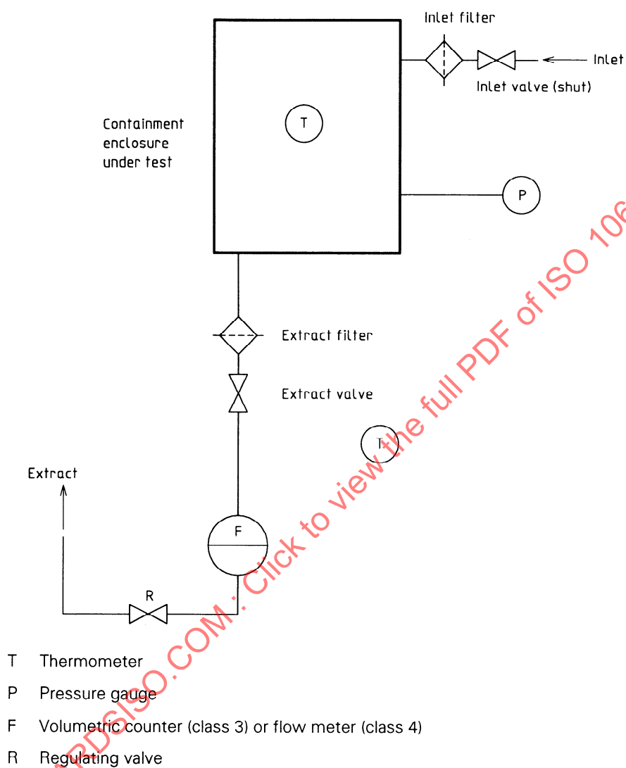
Figure 3 — Schematic diagram of the measuring system for the constant pressure method (containment enclosure kept at a negative pressure)
