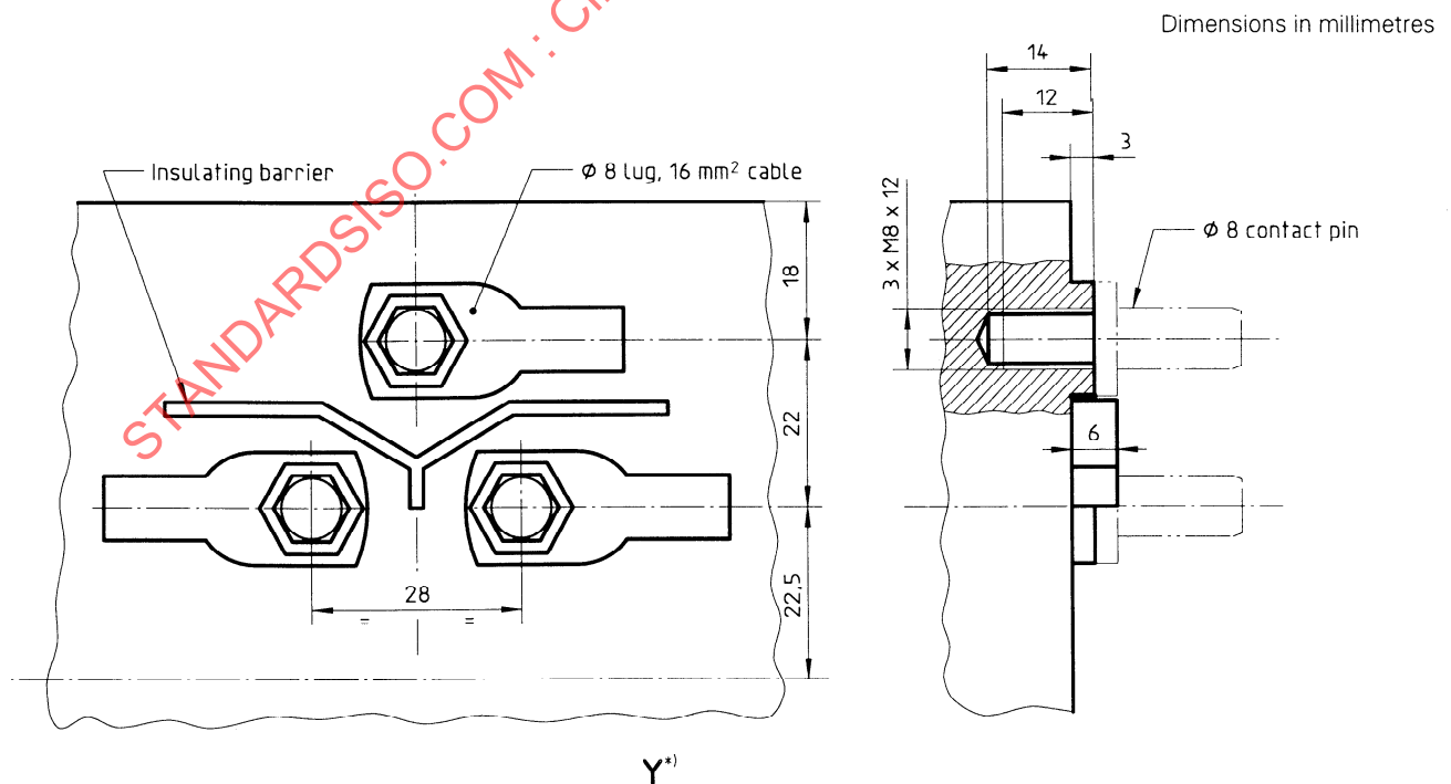
Figure 3 — Dimensions of type J transformers
