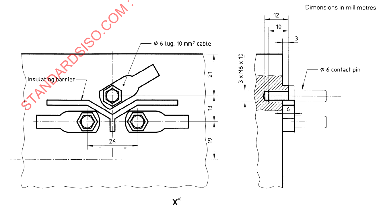
Figure 2 — Size and location of the 3 M6 holes intended for supply connection of type H transformers
