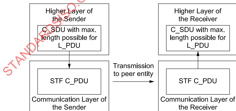
Figure 8 — Example of unsegmented message
