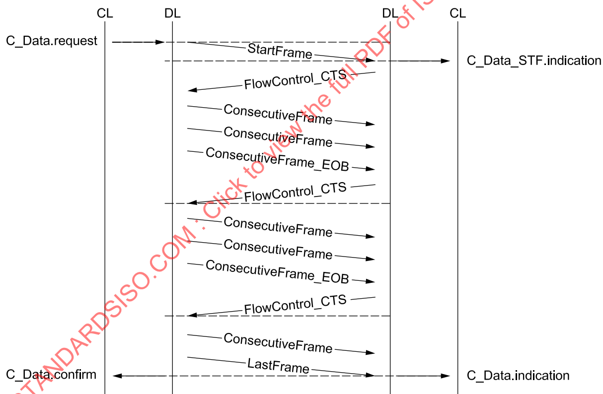
Figure 3 — Example of segmented unacknowledged message (known message length)
