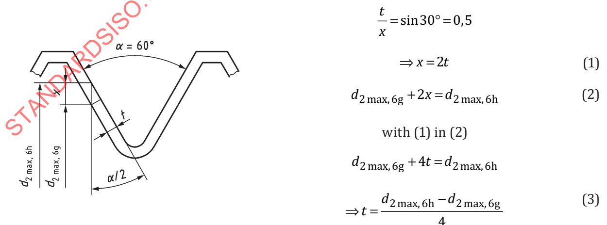
Figure B.1 — Geometrical relationship between coating thickness and pitch diameter
