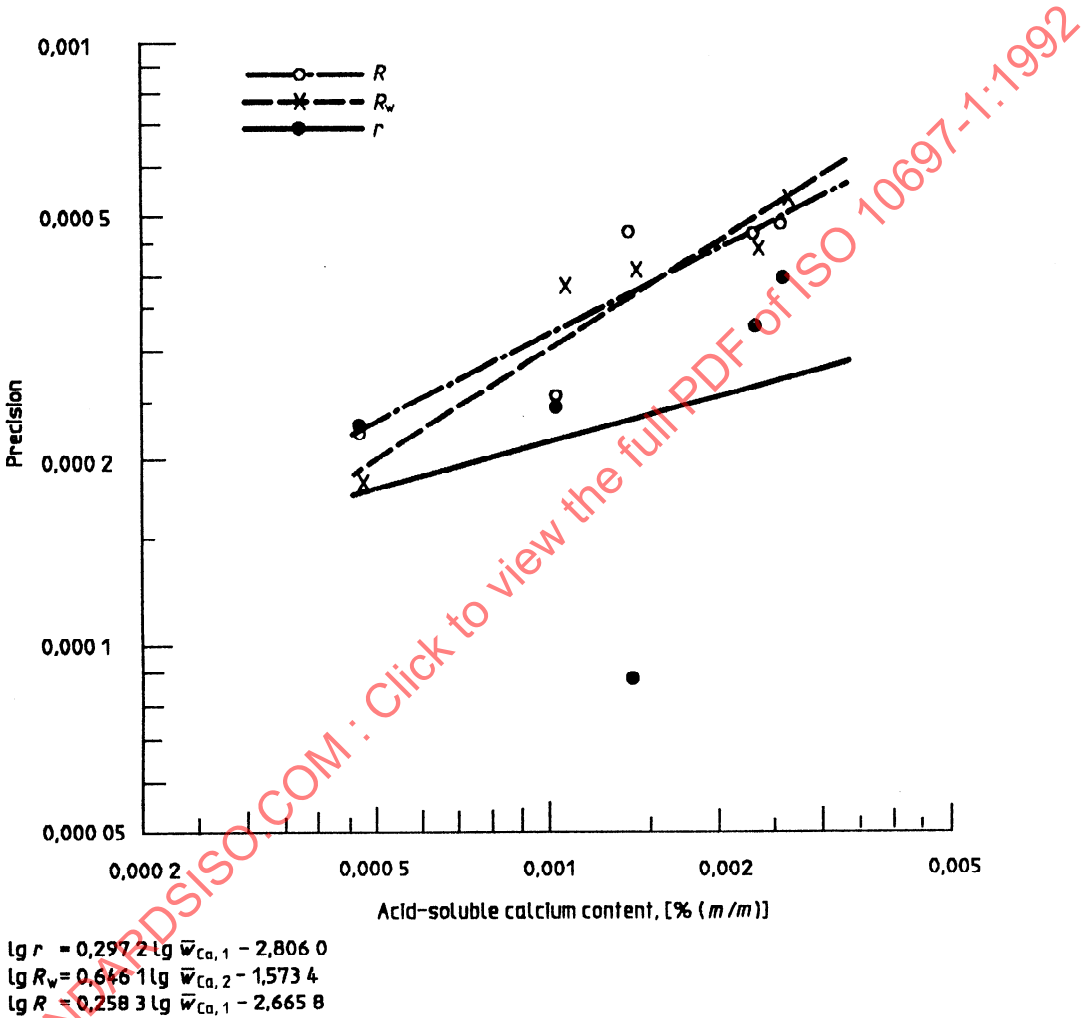
Figure C.1 — Logarithmic relationship between acid-soluble calcium content ( w_{Ca} ) and repeatability ( r ) or reproducibility ( R and R_w )
