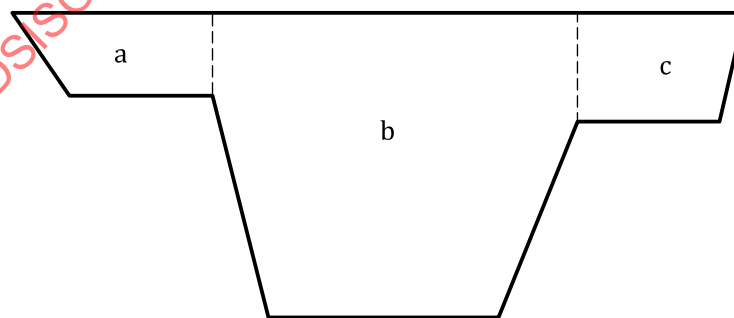
Figure 3 — Composite cross section of a main channel and floodplain
