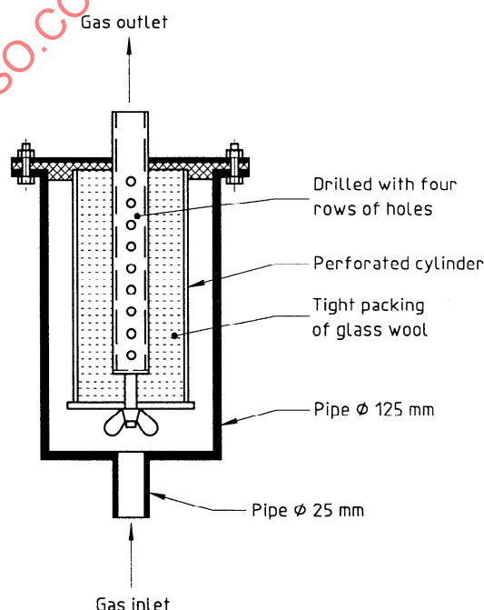
Figure 6 — Separator
