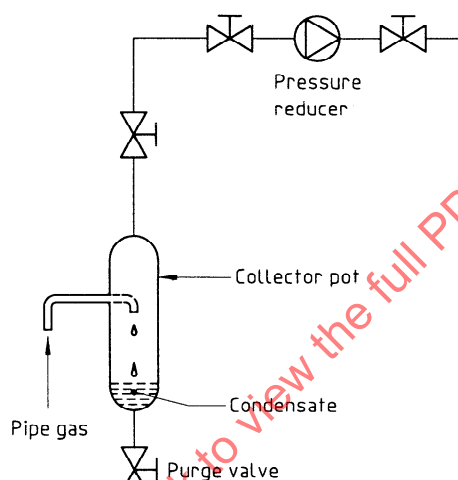
Figure 5 — Drip pot installation
