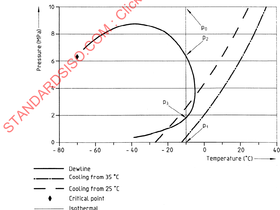
Figure 2 — Example of a pressure/temperature diagram for natural gas
