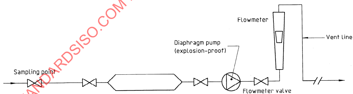
Figure C.3 — Sampling into glass cylinders from a sub-atmospheric pipeline
