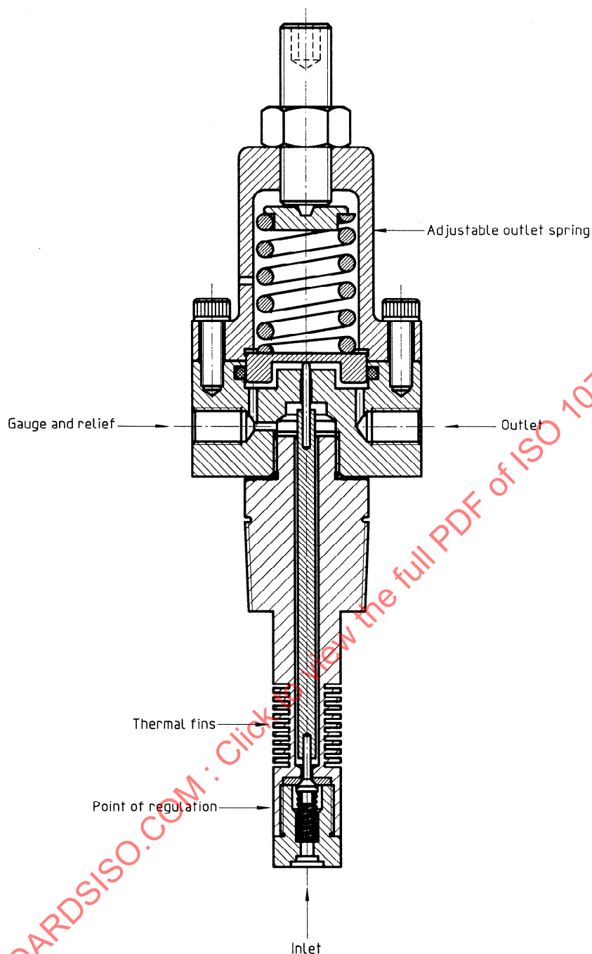
Figure 4 — Regulated probe
