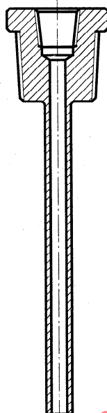
Figure 3 – Straight-tube probe
