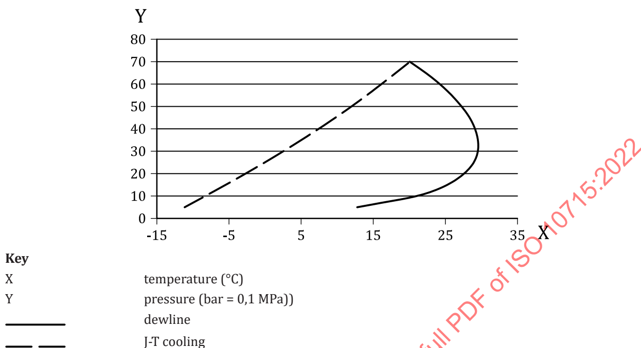
Figure E.2 — Phase behaviour of methane/nonane mixture
