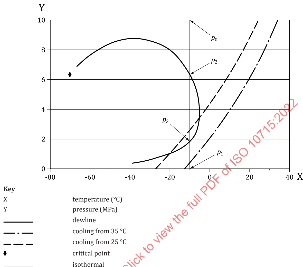
Figure 8 — Example of a pressure/temperature diagram for natural gas
