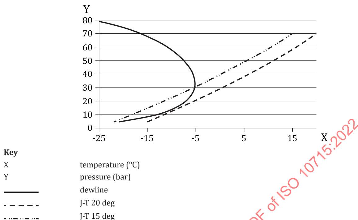
Figure E.3 — Phase behaviour of real natural gas
