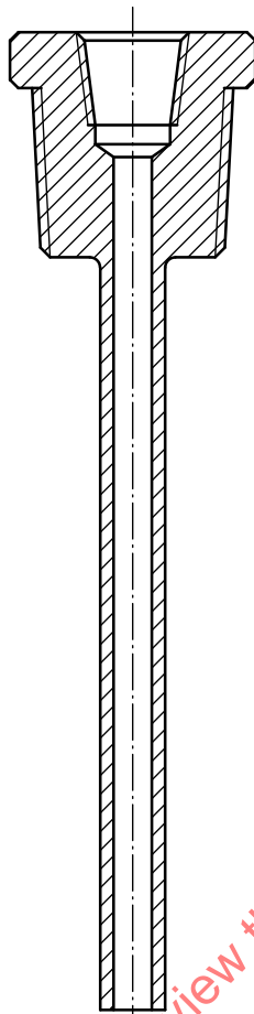
Figure 9 — Straight-tube probe
