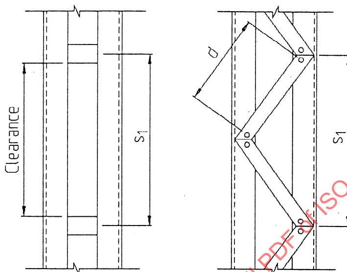
Fig. A.8.4.6.b Spacing of built up members
