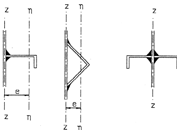
Fig. 8.6.5.1.c Types of stiffeners
