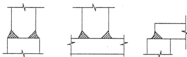
Fig. 8.9.6.2 Partial penetration groove welds
