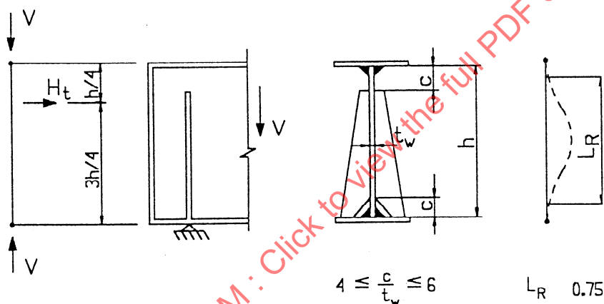
a) Calculation model for end stiffeners
