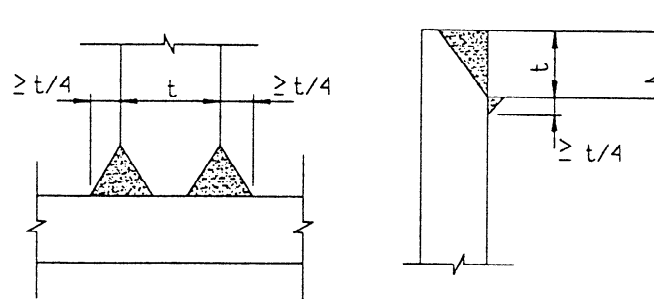
Fig. 8.9.7.10 Reinforcement for T- and corner joints
