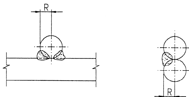
Fig. 8.9.7.11.b Flare grooves in solid section joints
