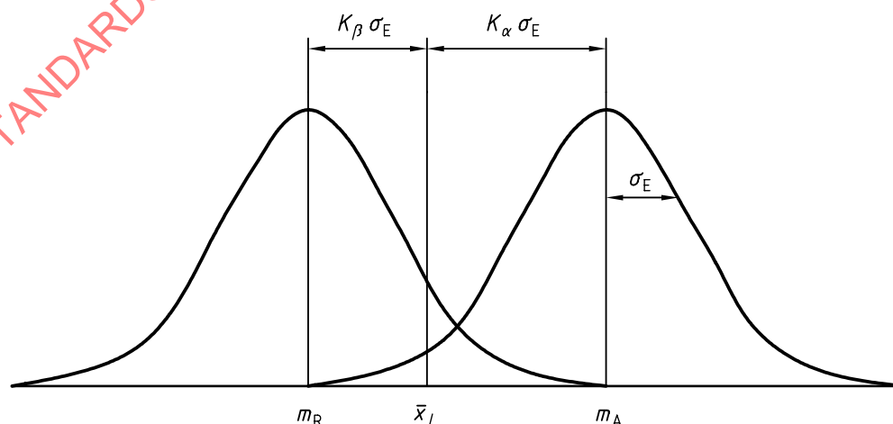
Figure C.1 — Relationship between m_A , m_R and acceptance value (Distribution of \bar{x}_{...} ; lower specification limit)
