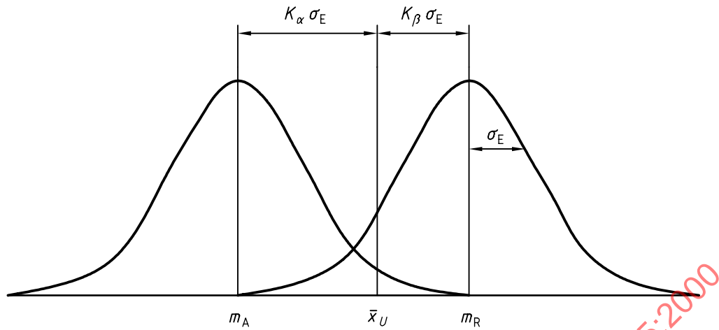
Figure C.2 — Relationship between m_A , m_R and acceptance value (Distribution of \bar{x} ; upper specification limit)
