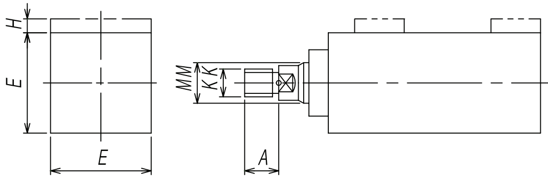
Figure 1 — Basic dimensions
