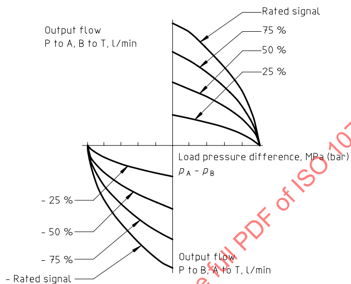
a) Output flow versus load pressure difference
