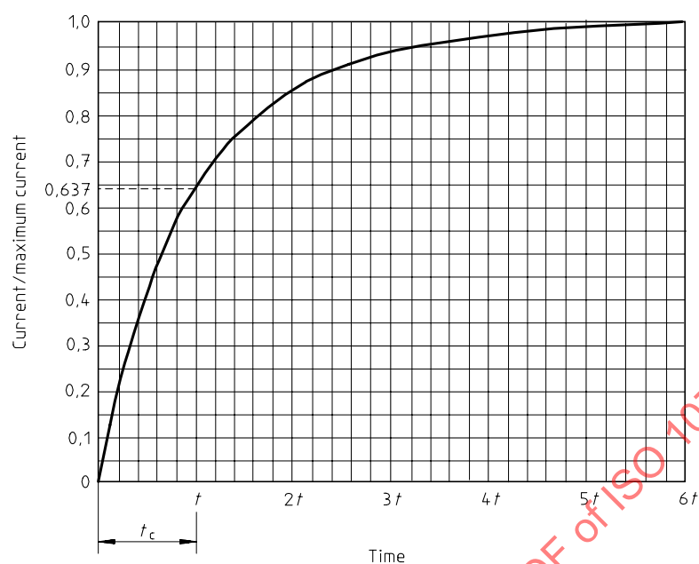
Figure 4 — Valve coil step response
