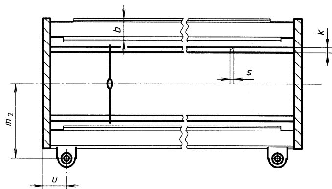
Figure 6 — Bushes outside lower frame stave
