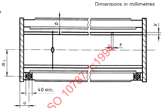
Figure 4 — Bushes inside lower frame stave
