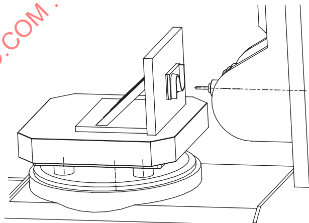
c) Machining centre with a tilting head and a rotary table
