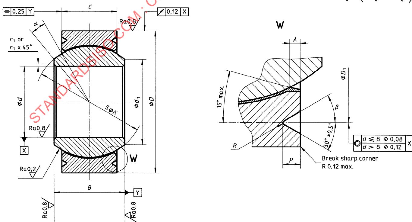
Figure 2 — Spherical plain bearing with self-lubricating liner with face groove
