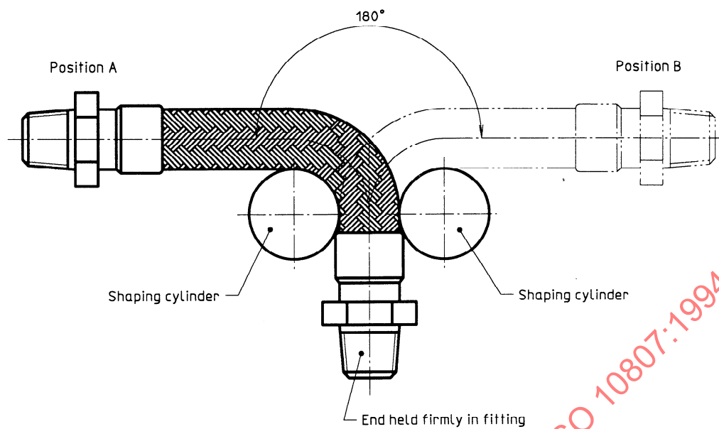
Figure B.1 — Flexural strength test
