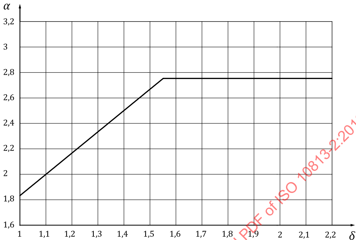
Figure A.7 — Relationship between the factor \alpha and the frame dimension ratio L_{fr}/B_{fr}
