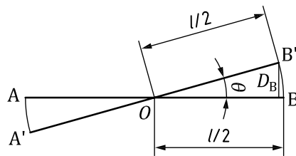
Figure 14 — Illustration of angular motion
