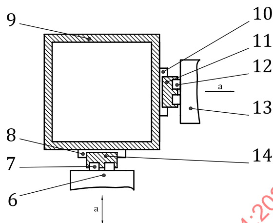
b) Top view of bi-axial system
