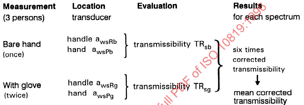
Figure 7: Principle of determination of mean corrected transmissibility
