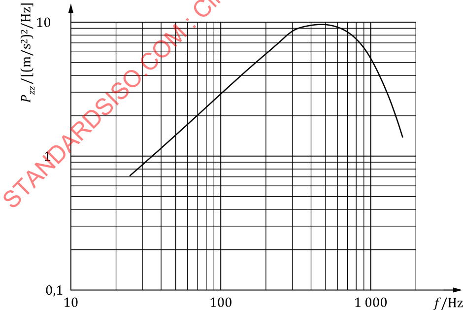
Key P_{zz} accelerometer power spectral density f frequency
