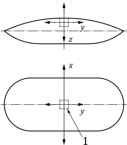
Key 1 accelerometer location x, y, z three mutually orthogonal measurement axes
