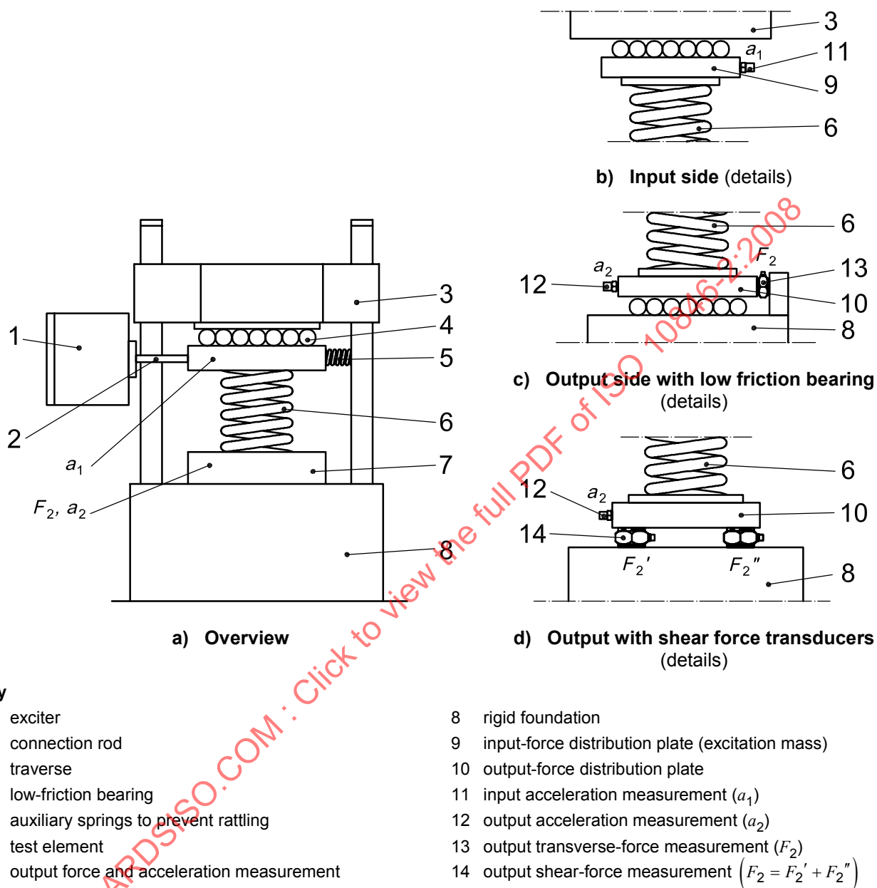
Figure 3 — Example 1 of laboratory test rig for measuring the dynamic transfer stiffness for transverse translation
