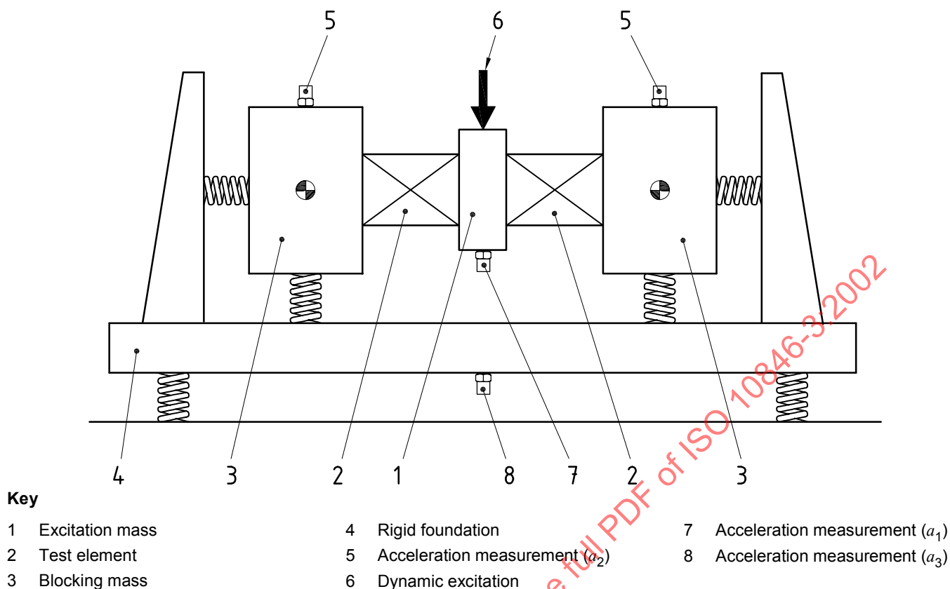
Figure 6 — Example 2 of laboratory test rig for measuring the dynamic transfer stiffness for transverse translations
