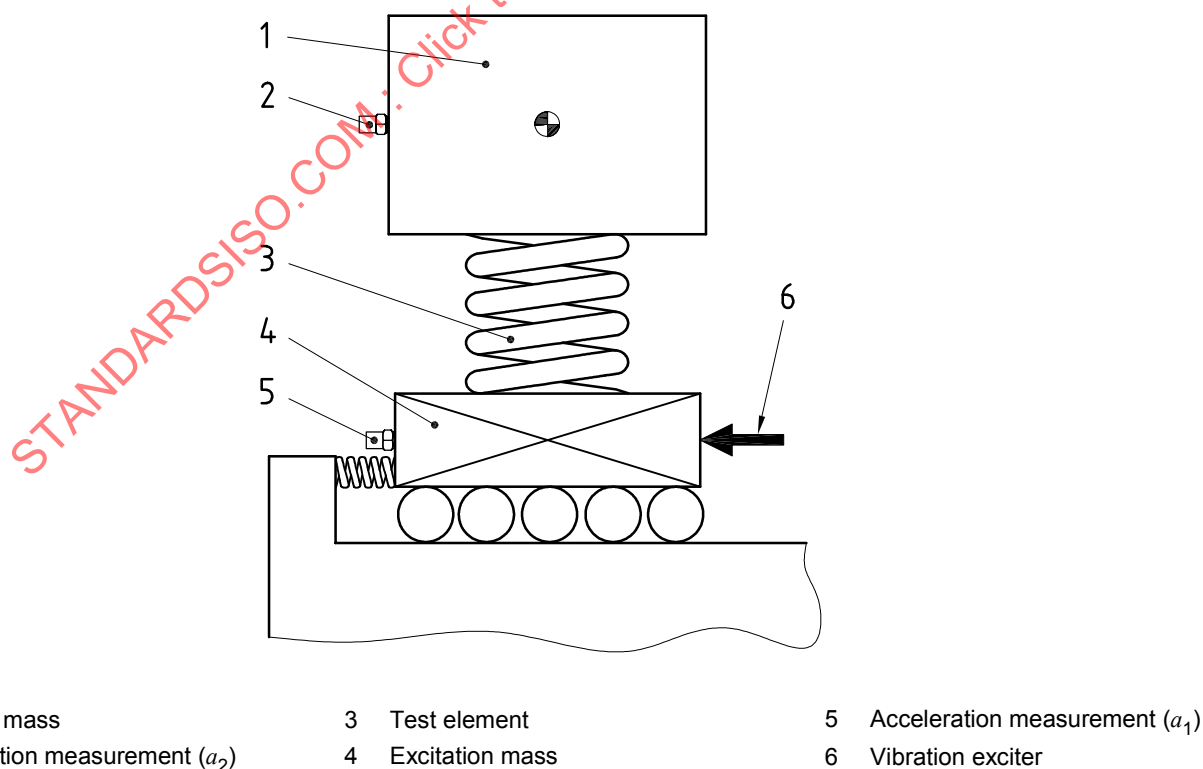
Figure 7 — Example 3 of laboratory test rig for measuring the dynamic transfer stiffness for transverse translations
