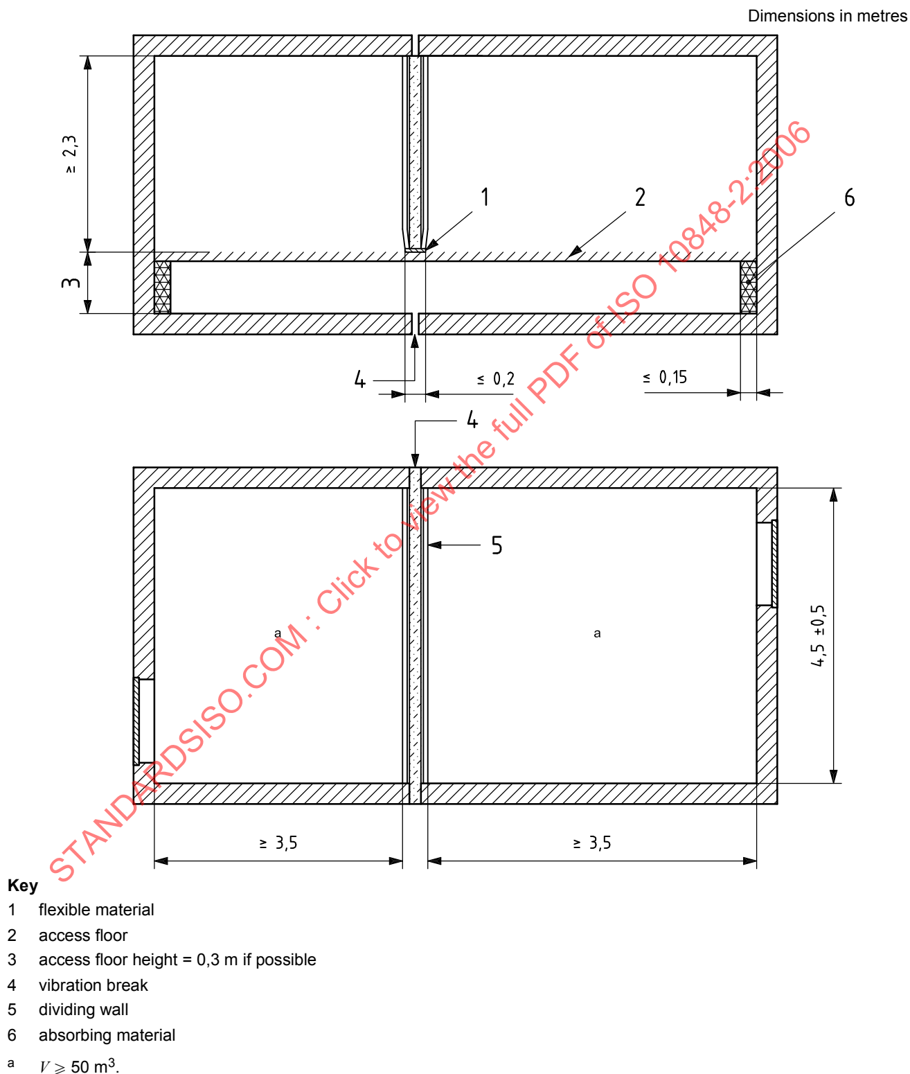
Figure 1 — Requirements for the dimensions of the laboratory and for the mounting of the access floor and the dividing wall
