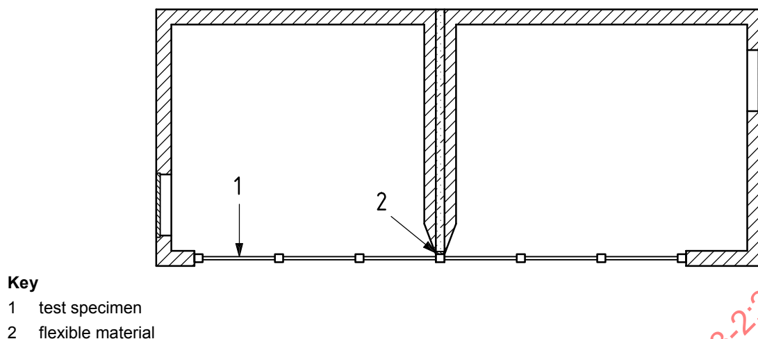
Figure 3 — Example of installation of a façade — Horizontal transmission (plan view)
