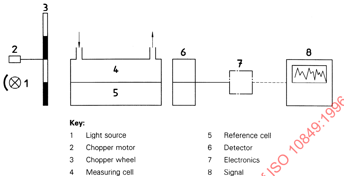
Figure 4 — Example of a NDIR analyser
