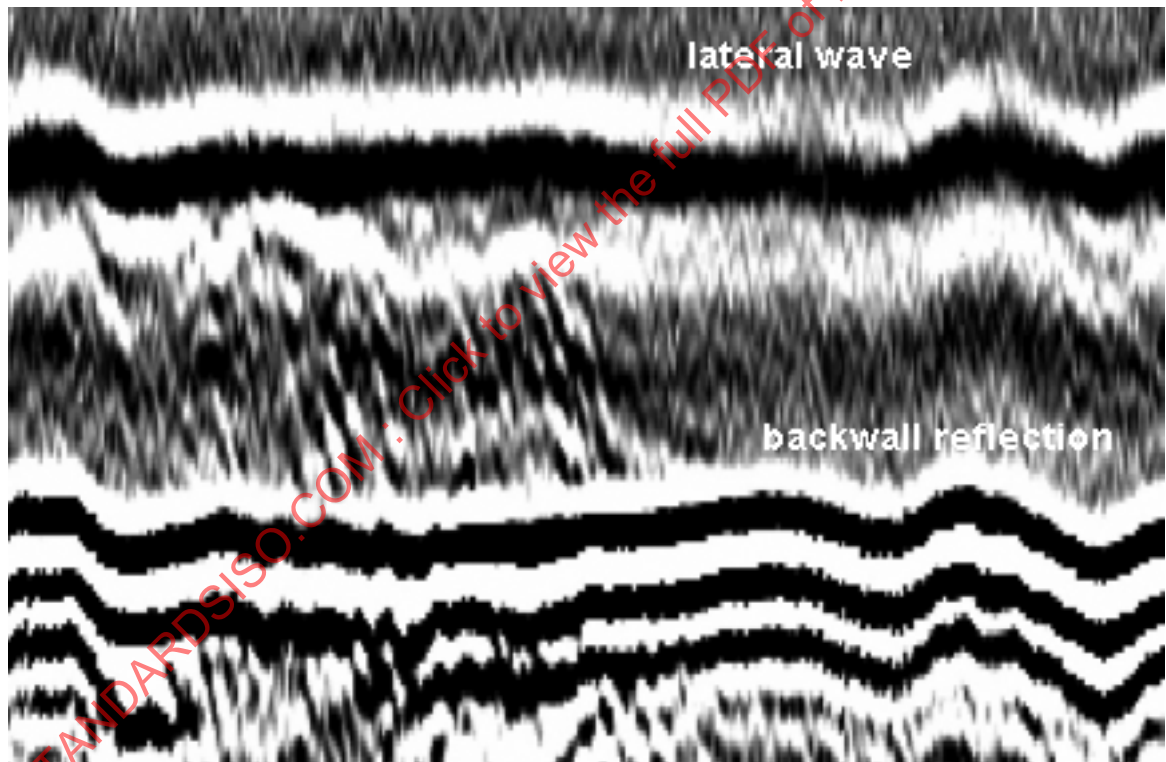
Figure B.2 — Gain setting too low
