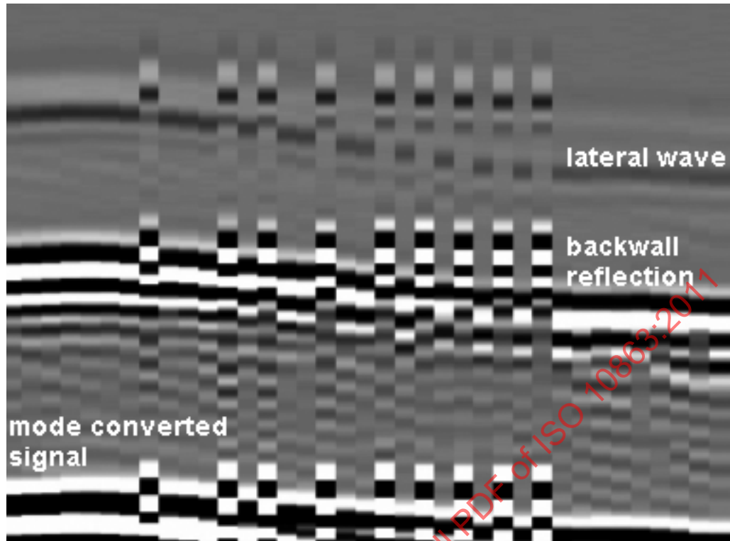
Figure B.6 — Time base triggering problems
