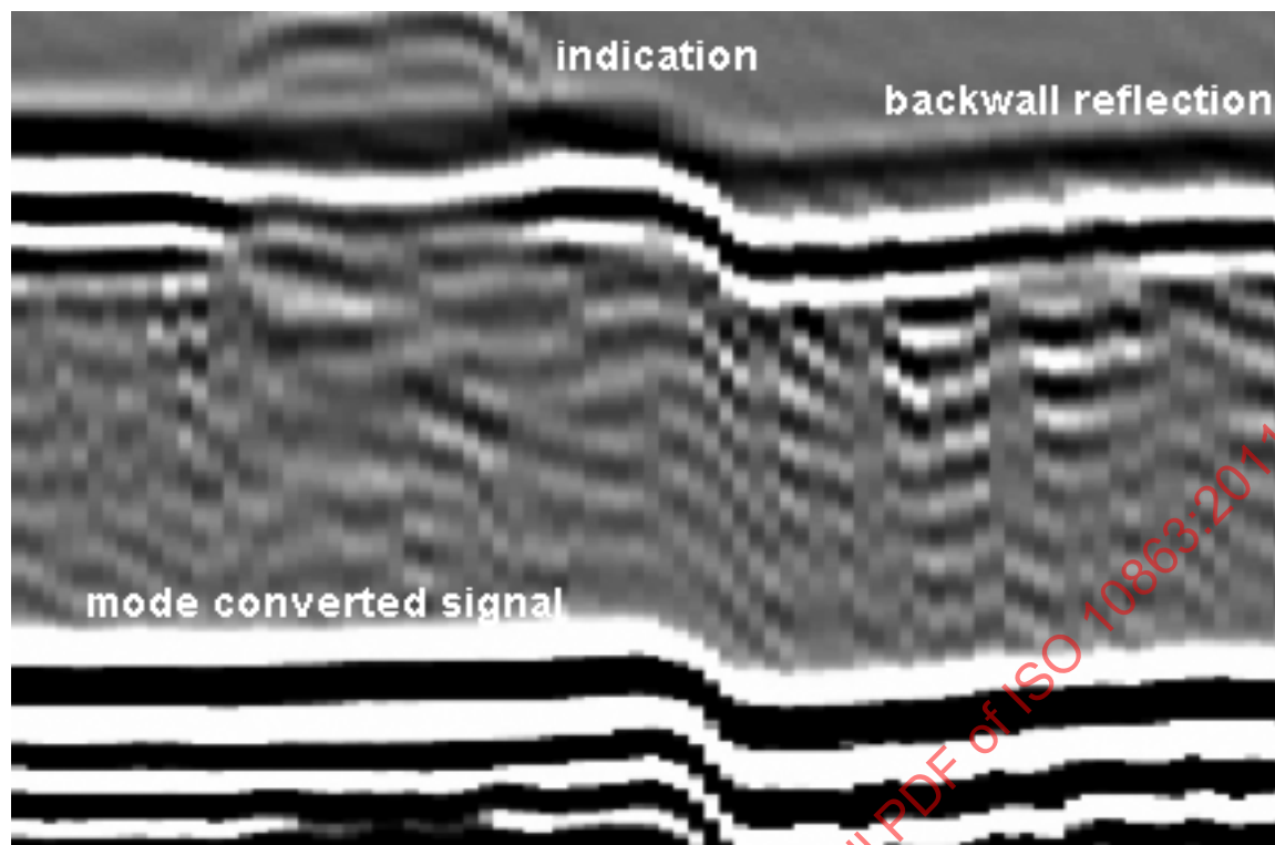
Figure B.4 — Inappropriate time window setting
