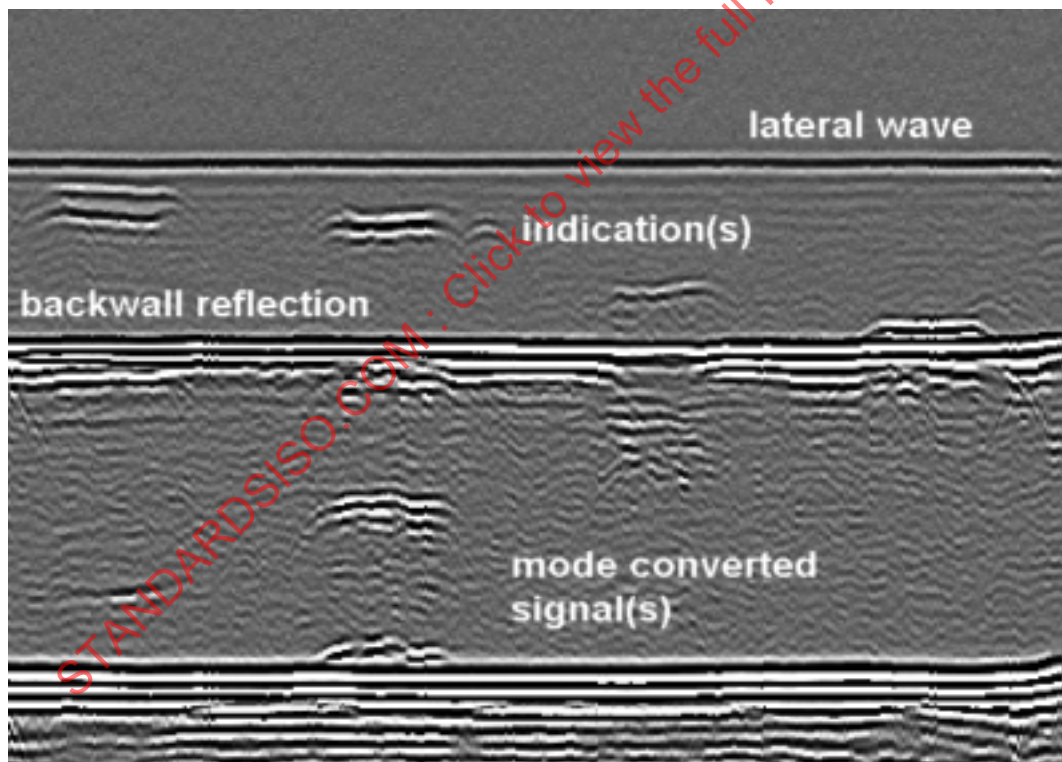
Figure B.1 — Satisfactory TOFD image
