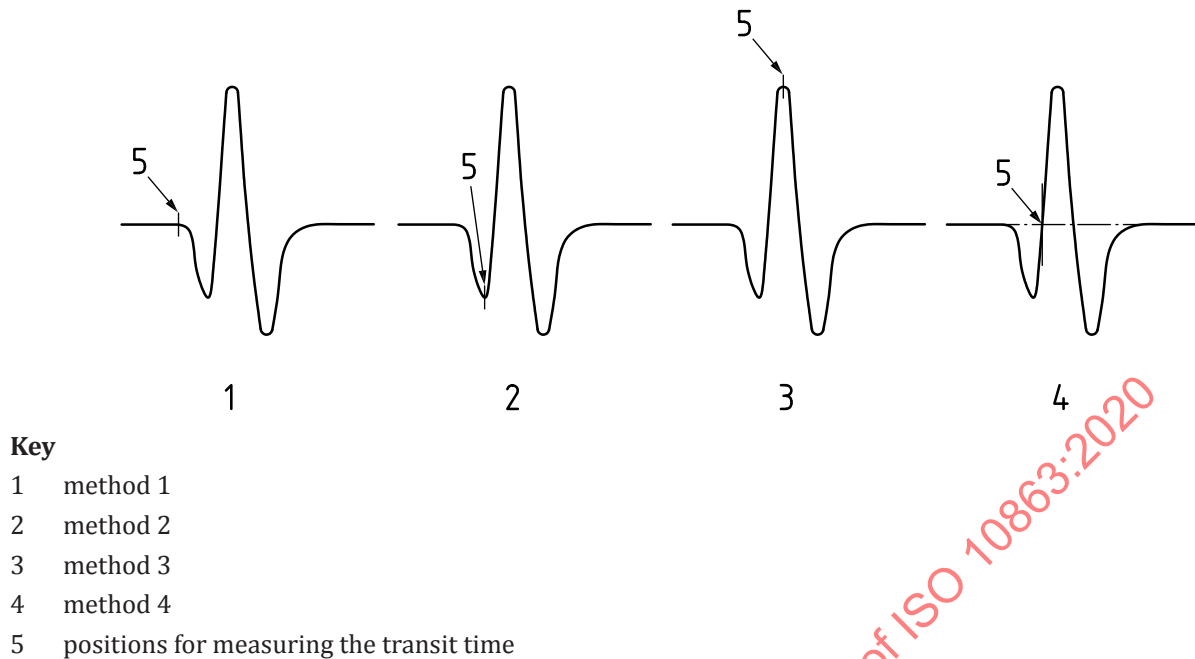
Figure 6 — Positions of the cursor for time measurements — Methods 1, 2, 3 and 4
