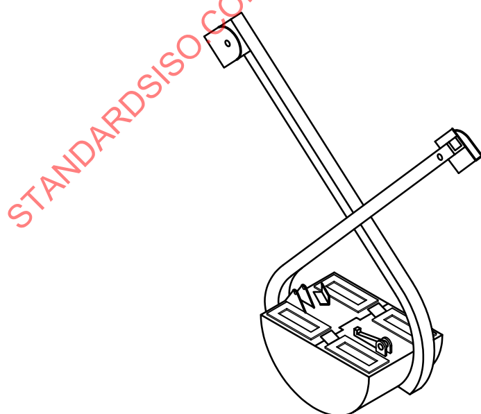
Figure 8 — The Van Veen grab (closed position)
