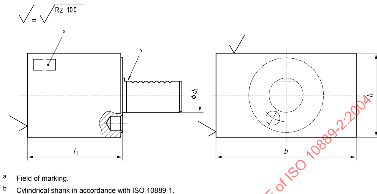
Figure 1 — Type A1 tool holder, rectangular
