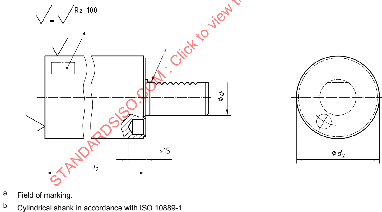
Figure 2 — Type A2 tool holder, round
