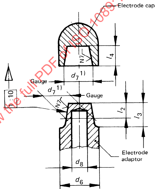
Type C for electrode caps
