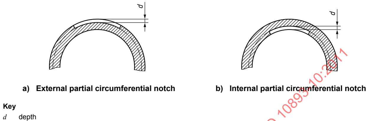
Figure 2 — Typical transverse notches
