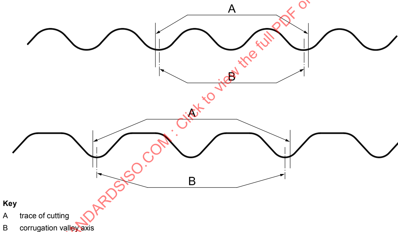
Figure 4 — Longitudinal cutting of specimens
