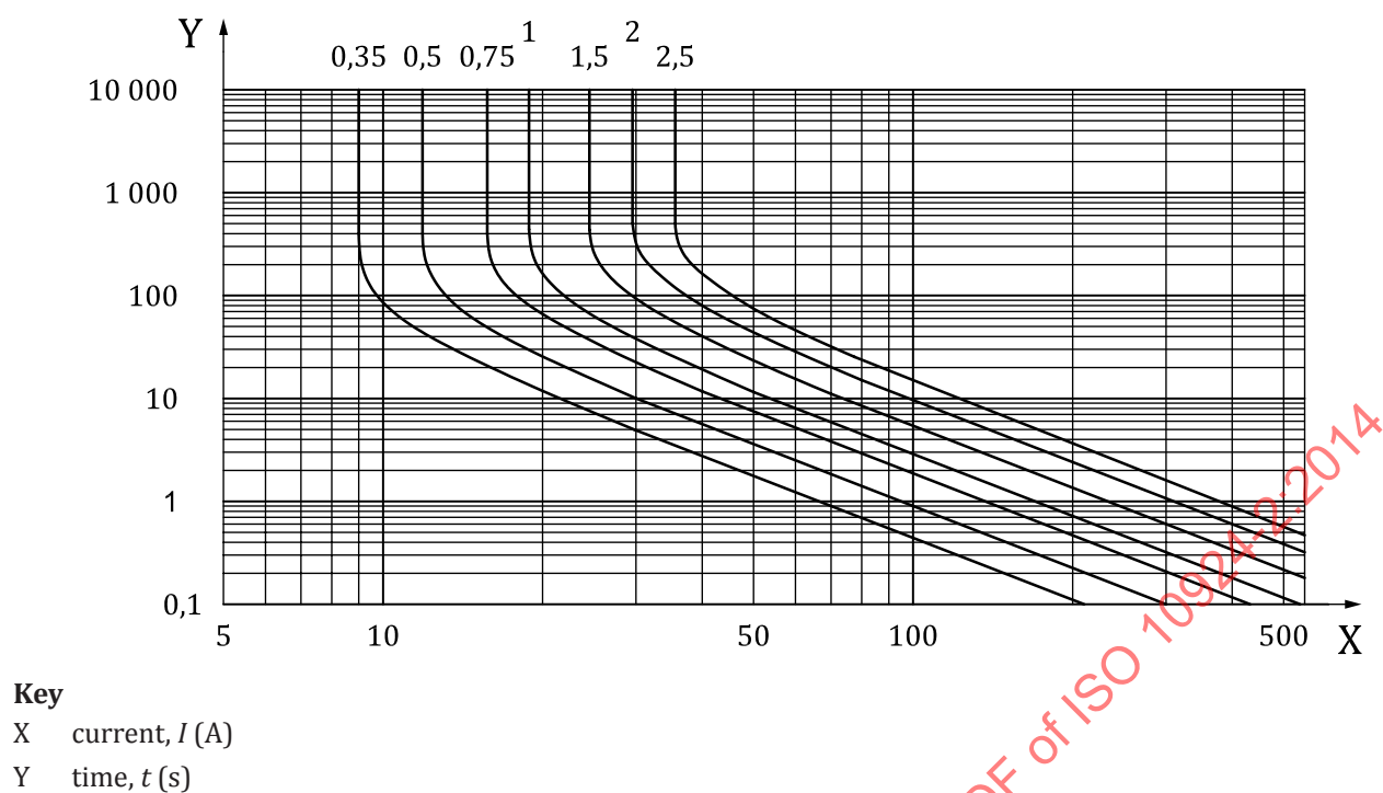
Figure A.5 — Example of I - t - characteristics of conductors
