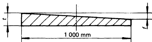
FIGURE 3 – Parallelism
