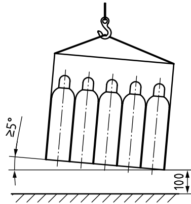
Figure 2 — Vertical drop test arrangement
