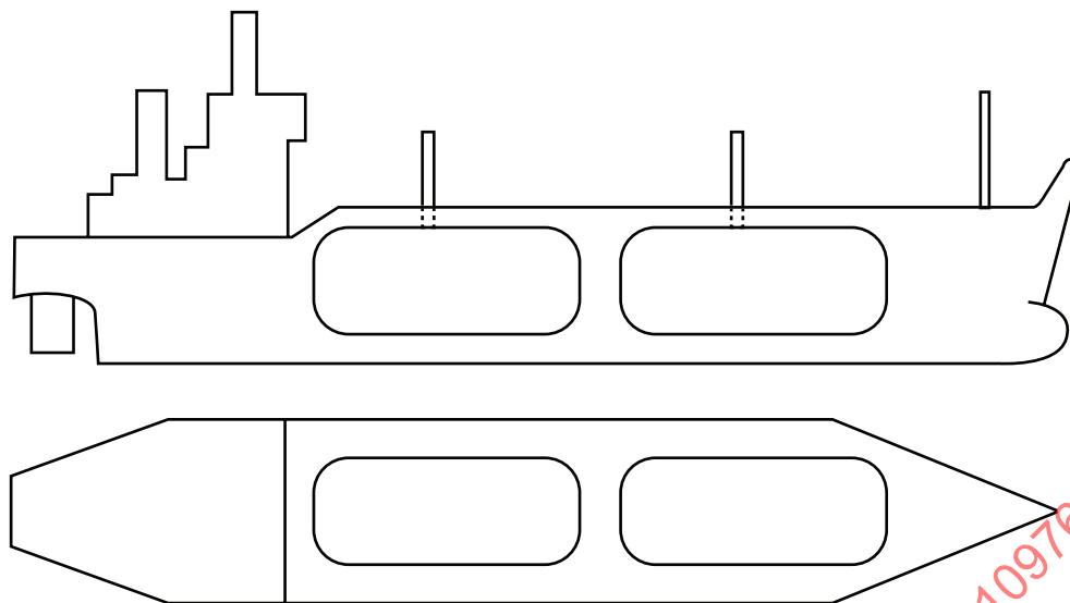
Figure A.4 — Vessel with IMO Type C tanks
