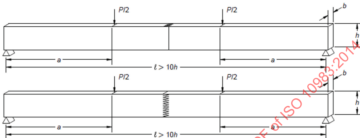
Figure A.4 — Edgewise bending with four-point loading
