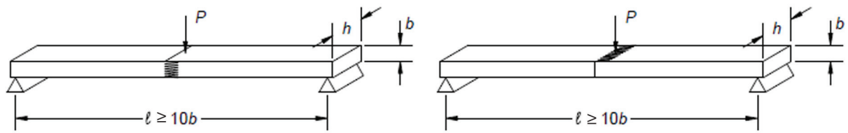
Figure A.1 — Flatwise bending with three-point loading
