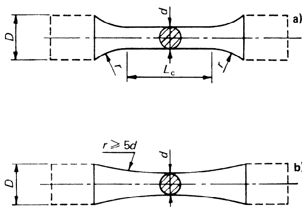
FIGURE 1 — Test pieces of circular cross-section
