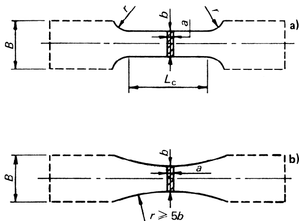
FIGURE 2 — Test pieces of rectangular cross-section
