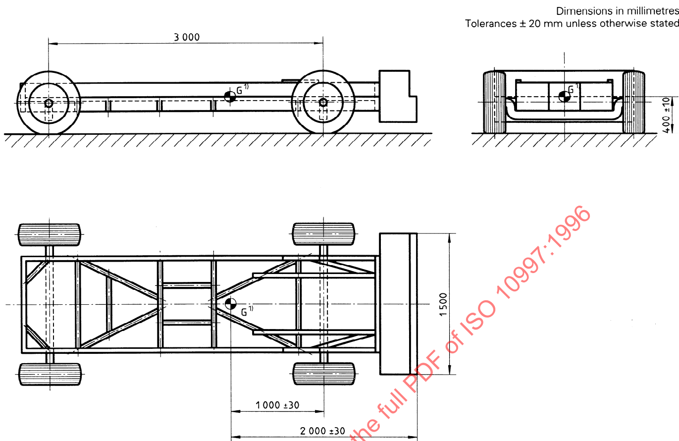
Figure 4 — Example of MDB carriage
